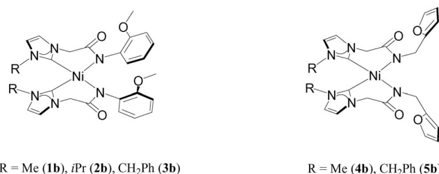
Figure 1. Nickel complexes of the amido-functionalized N-heterocyclic carbene, 1b–5b .
