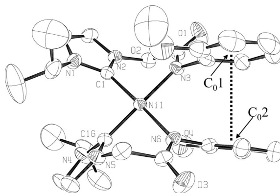
Figure 4. Offset or slipped \pi – \pi interaction observed in 2b displaying a centroid(C 01 )-to-centroid(C 02 ) distance of 3.926 Å.
