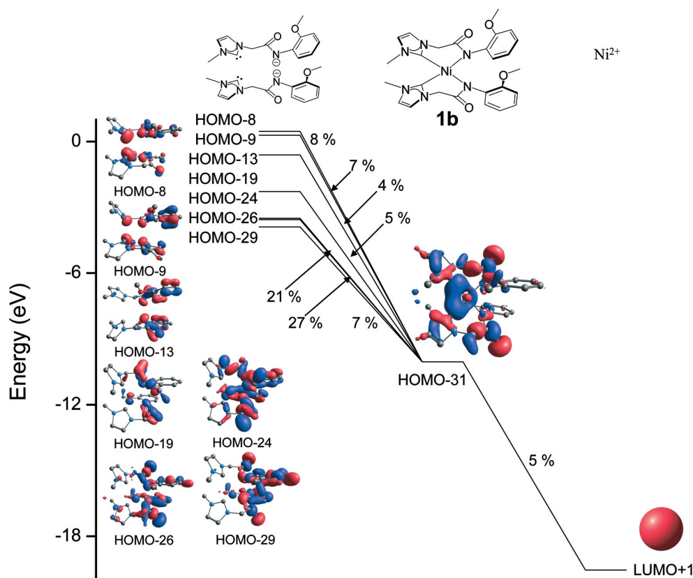
Figure 6. Simplified orbital interaction diagram showing the major contributions of the NHC–nickel bond in 1b .
