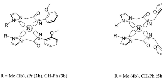
Figure 5. Interaction of the filled carbene lone pairs and the amido groups of the free NHC ligand fragments with the unfilled 4s orbital of nickel in 1b–5b .
