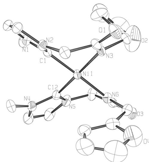
Figure 3. ORTEP diagram of 4b . Selected bond lengths (Å) and angles (°): Ni1–C1 1.852(4), Ni1–C12 1.859(4), Ni1–N3 1.921(3), Ni1–N6 1.938(3), C1–Ni1–C12 93.68(16), C1–Ni1–N3 86.59(14), C12–Ni1–N6 87.35(14), N3–Ni1–N6 92.56(13).
