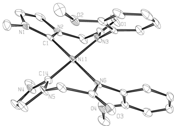
Figure 2. ORTEP diagram of 1b . Selected bond lengths (Å) and angles (°): Ni1–C1 1.959(3), Ni1–C14 1.742(2), Ni1–N3 1.8564(19), Ni1–N6 2.052(2), C1–Ni1–N3 86.49(9), C14–Ni1–N6 86.42(10), C1–Ni1–C14 93.01(11), N3–Ni1–N6 94.07(9).
